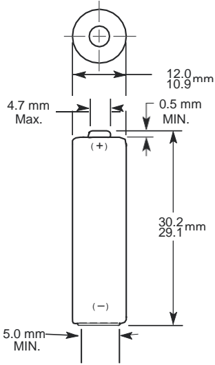
Dimensions shown are IEC/ANSI standards
