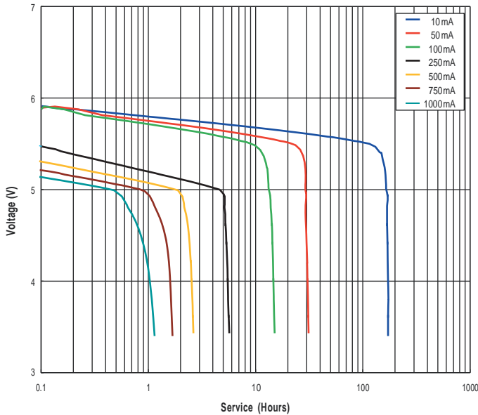
Continuous Discharge RT to 3.4Volts
